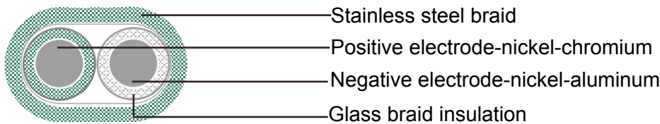
KX glass braid insulated
